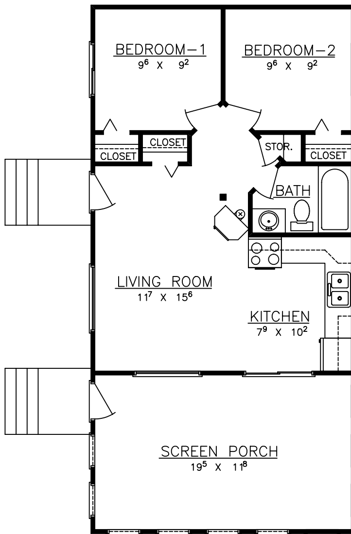
FLOOR PLAN
